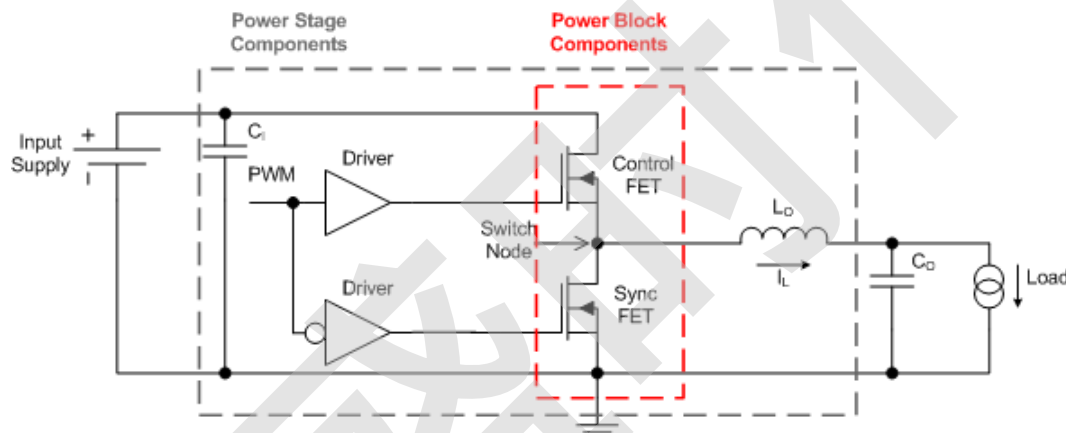
Figure 28. Equivalent System Schematic
