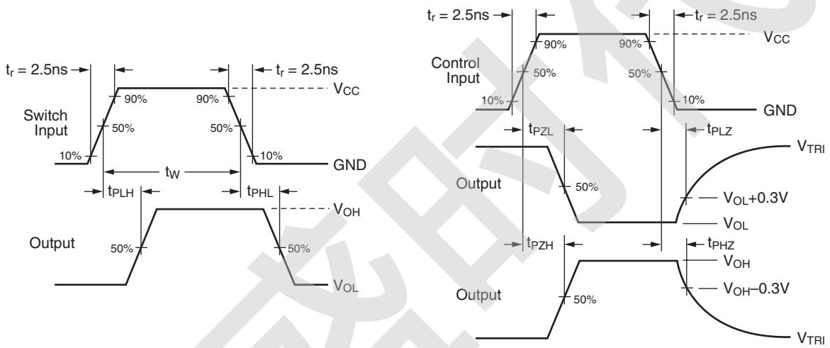
Figure 13. AC Waveforms
