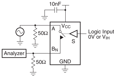
Figure 16. Off Isolation
