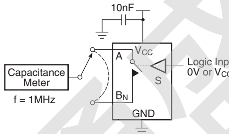
Figure 18. Channel Off Capacitance
