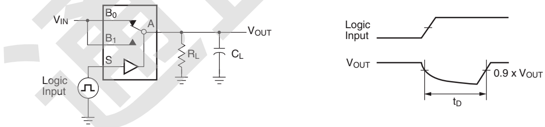
Figure 14. Break-Before-Make Interval Timing
