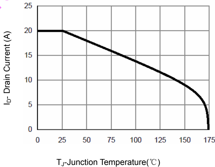
Figure 11 Current De-rating
