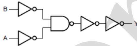
Figure 3. Logic diagram
