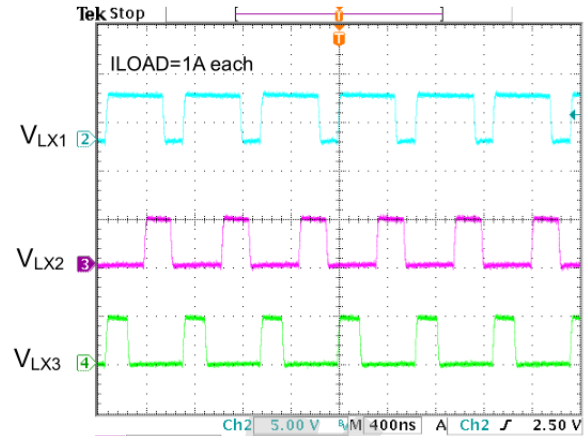
V LX1,2,3 Switching Waveform
