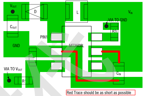
Figure 3. MT3608L Suggested Layout
