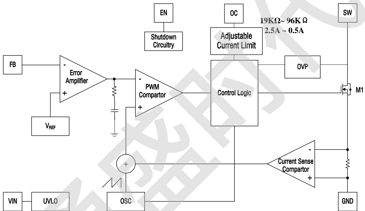
Figure 2. MT3608L Block Diagram
